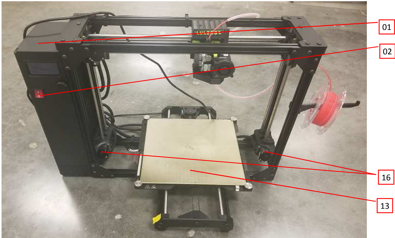
Photo 1 - External front view of TAZ Workhorse
