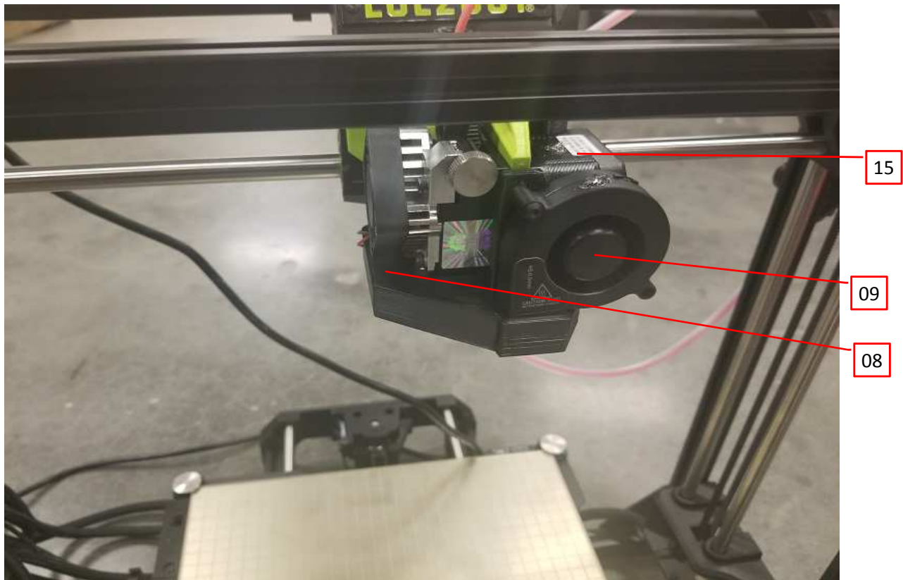
Photo 4 - Dispenser Head of TAZ Workhorse
