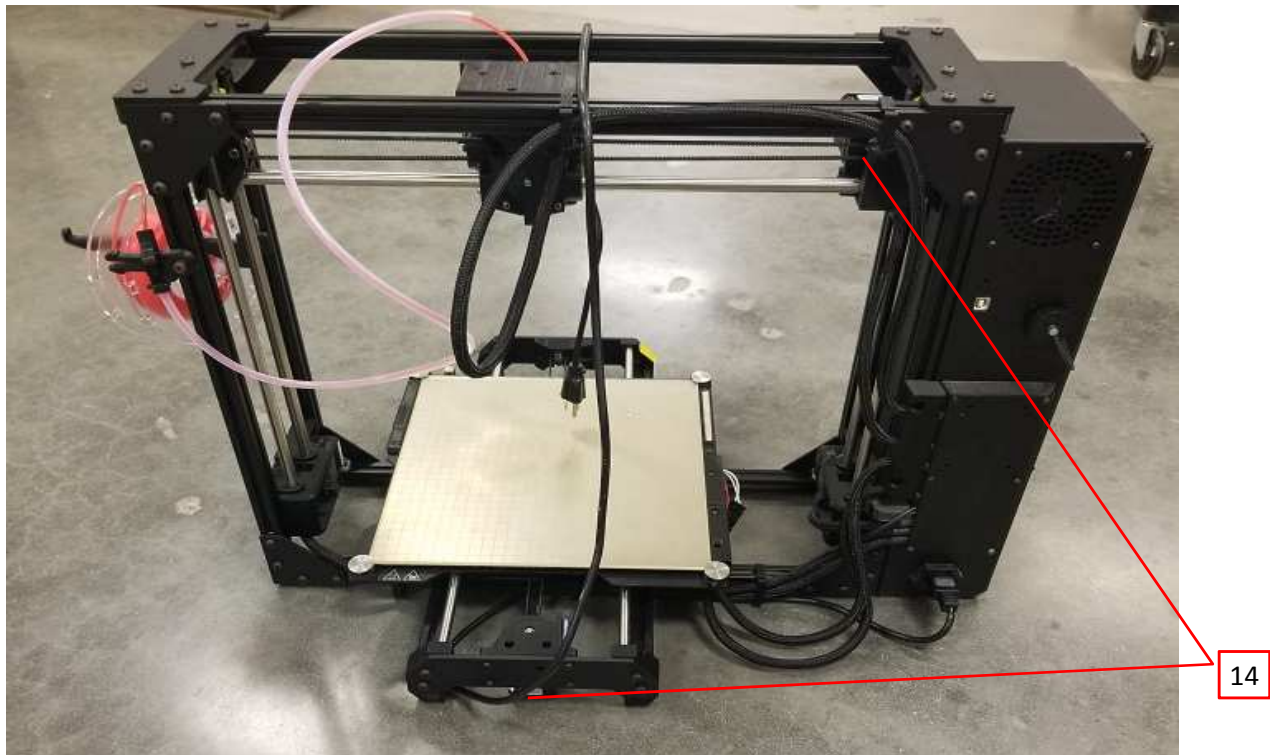
Photo 2 - External back view of TAZ Workhorse
